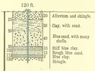
SECTIONS OF ARTESIAN WELLS at Napier, Havelock, and Clive, showing irregular bedding on the Heretaunga Plain.
